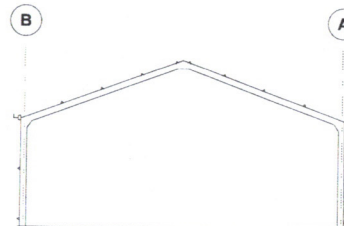
SECTION GRID 2
