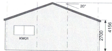
ELEVATION GRID 4
