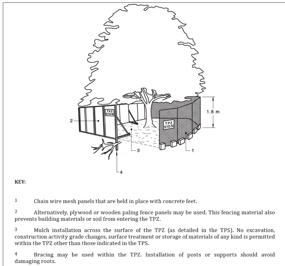
Figure 4- Detail of Tree Protection Fencing (AS 4970-2025)
