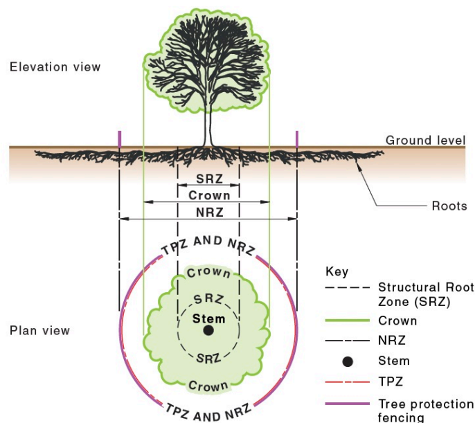
Figure 2: Indicative Notional Root Zone, Structural Root Zone & Tree Protection Zone of a tree with no development within its NRZ (AS-4970-2025)
